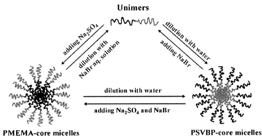
Fig. 2. Schematic illustration of the micellization behavior of the PMEMA- b -PSVPB diblock copolymer in aqueous solution at different conditions. Reprinted with permission from [32]. Copyright 2007 American Chemical Society.
